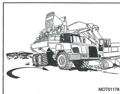
Figure 6.26 - Semicircular Loading
